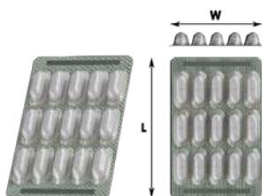
Blister plate 115x75mm (15 capsules) 2 blister plates per box
